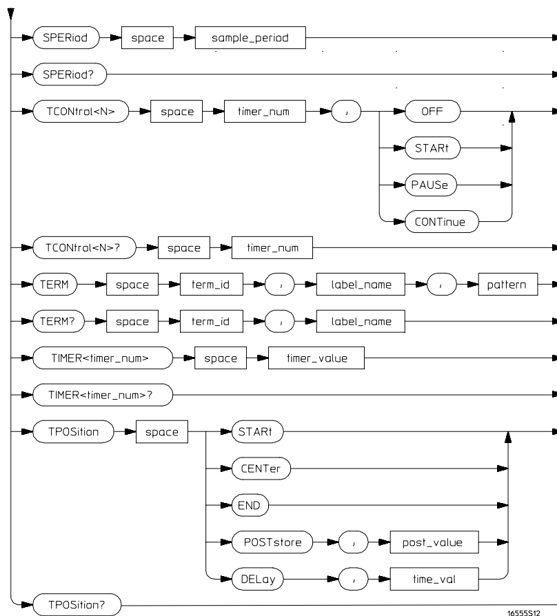
TTRigger Subsystem Syntax Diagram (continued)
